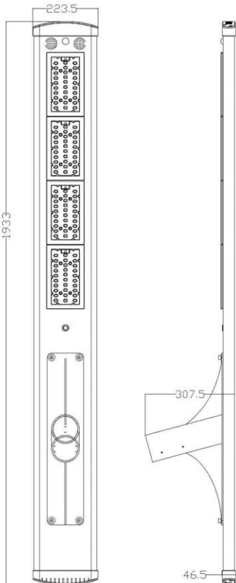
Simulation Drawing
