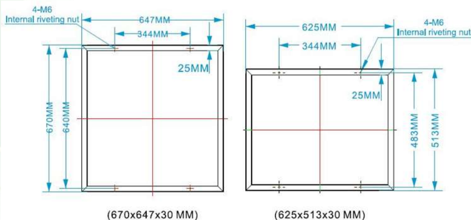
Solar Panel Dimension
