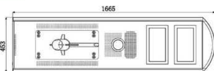
100W model diagram
